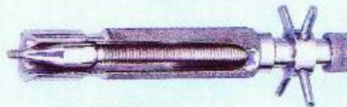
Cat. No. 662.00 Introducer/Extractor for Jewett Nail Plate
