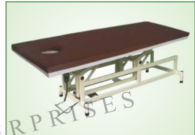
Code No : 194 Name : Massage Table (Up-Down Adjustable Base Frame) Size : 78"x30"x32" Made of : M.S. Powder Coated
