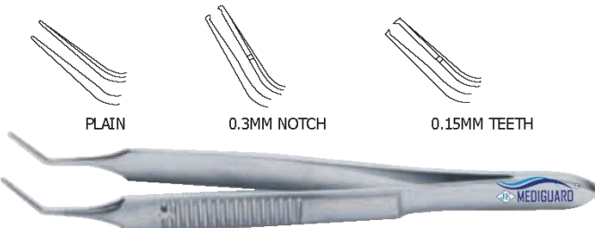
Mc PHERSON TYING FORCEPS 7MM ANGLED JAWS
